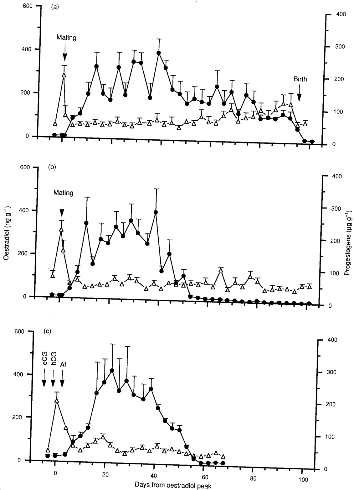
Fig. 1. Mean ( \pm SEM) faecal oestradiol ( \Delta ) and progesterone ( \bullet ) metabolite concentrations in (a) pregnant ( n=5 ) and (b) nonpregnant ( n=8 ) cheetahs after natural mating and in (c) nonpregnant cheetahs after induction of ovulation by gonadotrophin and artificial insemination (AI) ( n=6 ). Data are aligned to the oestradiol peak (day 0).
